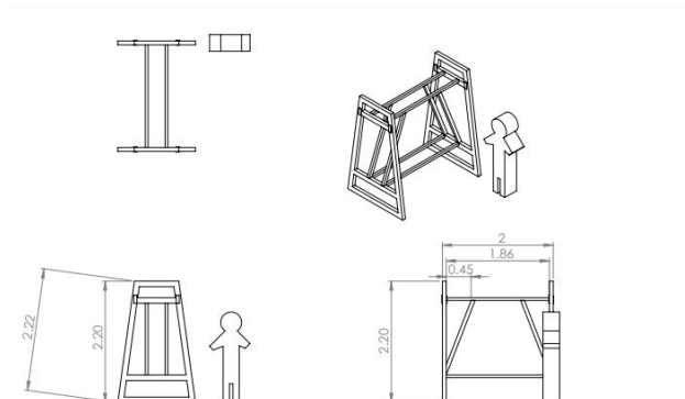
Figure 1 Desing of A-Frame for worker without climbing stairs
