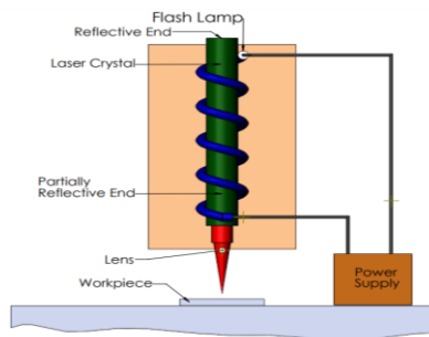
Figure 1. The Schematic of Laser Beam Machining
