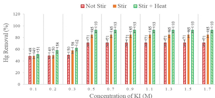
Figure 2. Removal of \text{Hg}^0 from carbon steel at different concentrations of KI (0.1 M–1.7 M) and 0.2 M \text{I}_2 after 16 h of reaction
