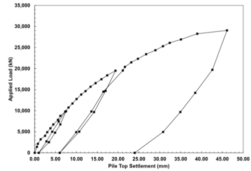
Figure 8. Load displacement curve for test pile A
