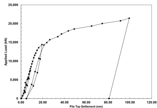
Figure 14. Load displacement curve for test pile C
