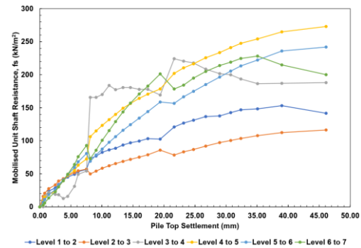
Figure 9. Mobilised unit shaft resistance for test pile A
