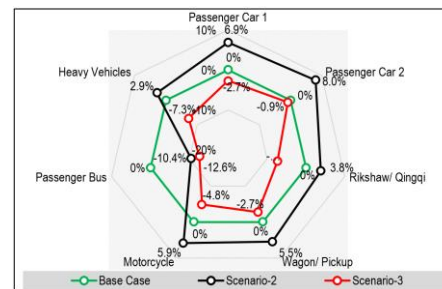
Figure 6. Percent change in delay based on vehicular classes
