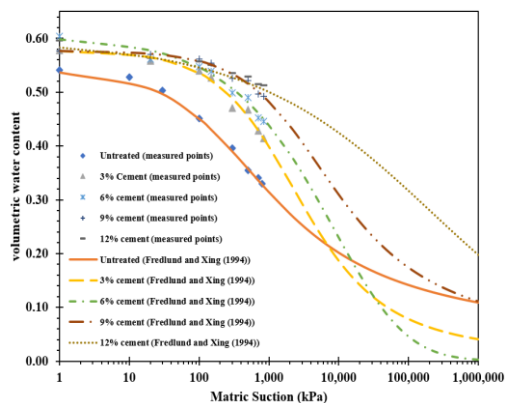
Figure 4. SWCC, according to measured and Fredlund Xing (1994) model
