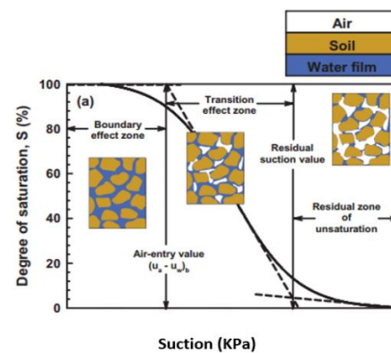
Figure 1. A typical SWCC (Oh and Vanapalli, 2011)
