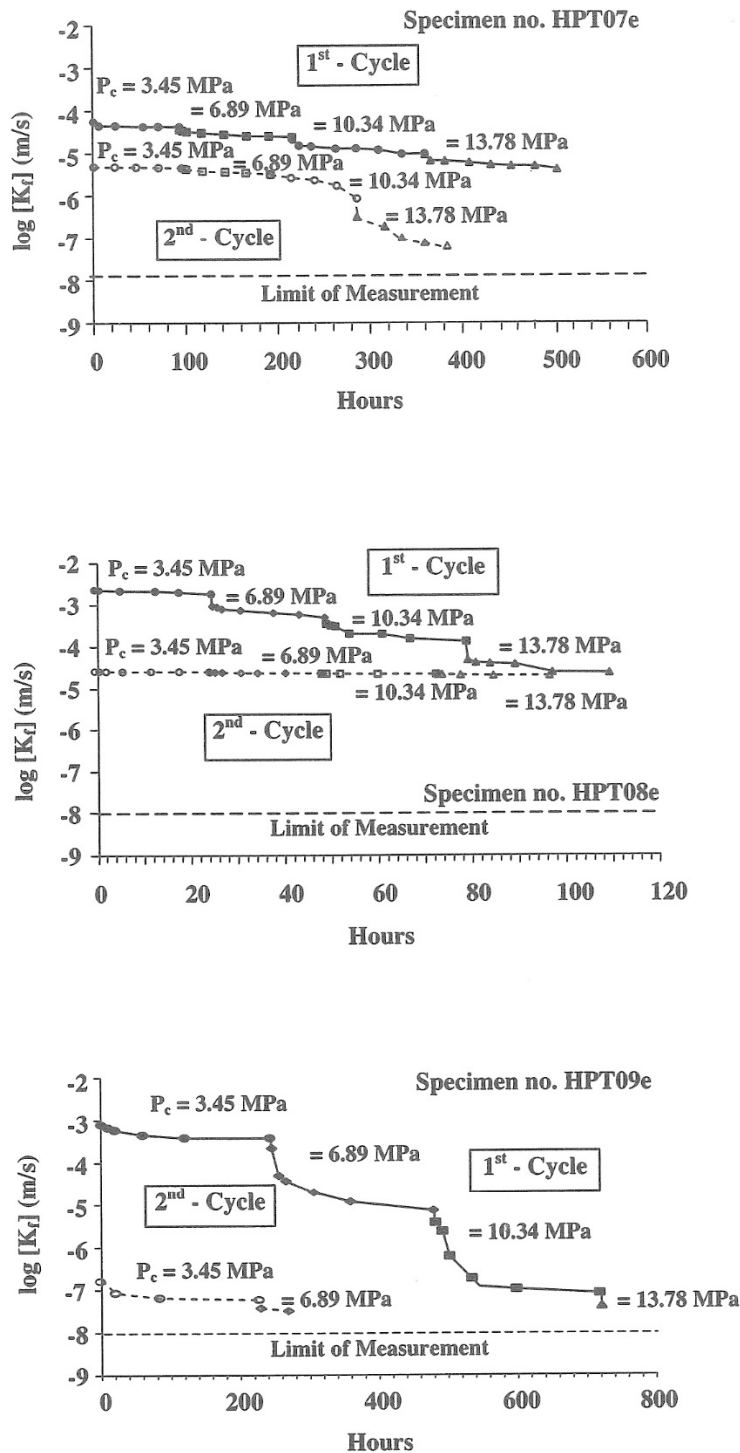
Figure 5. Hydraulic conductivity ( K_f ) of tension-induced fracture in three salt specimens as a function of time under quasi-static loading, for specimen *** HPT07e (top), HPT08e (middle) and HPT09e (Bottom)
