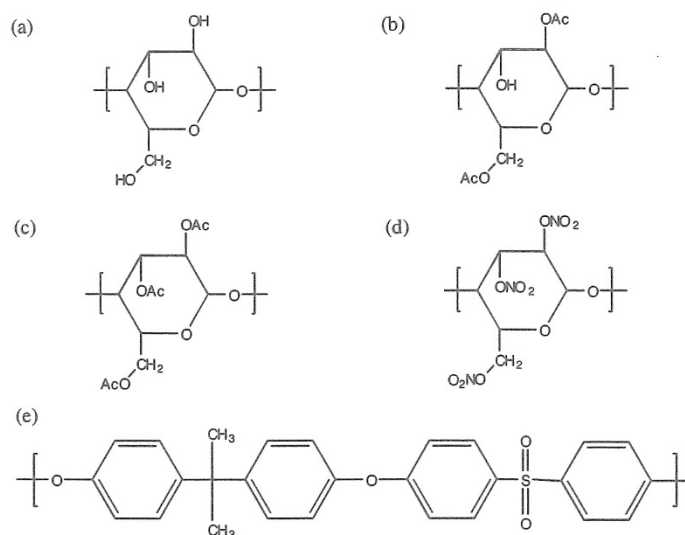
Figure 2. Chemical structures of the membrane materials. (a) Regenerated cellulose, (b) Cellulose acetate (about 70% of OH groups are acetylated), (c) Cellulose triacetate (more than 92% of OH groups are acetylated), (d) Cellulose nitrate, and (e) Polysulfone. (Some hydrogen atoms have been omitted for clarity)
