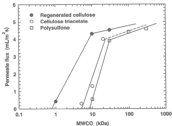
Figure 3. Initial permeate flux of mixed juice (prior to lime and heat treatment) through ultrafiltration membranes of various types
