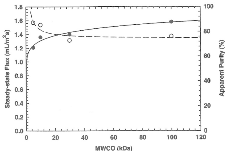
Figure 5. Steady-state membrane flux (●) and apparent purity of the permeate (○) for ultrafiltration of mixed juice (prior to lime and heat treatment) using regenerated cellulose membranes. Lines represent fits of the data taking into account boundary conditions at low MWCO
