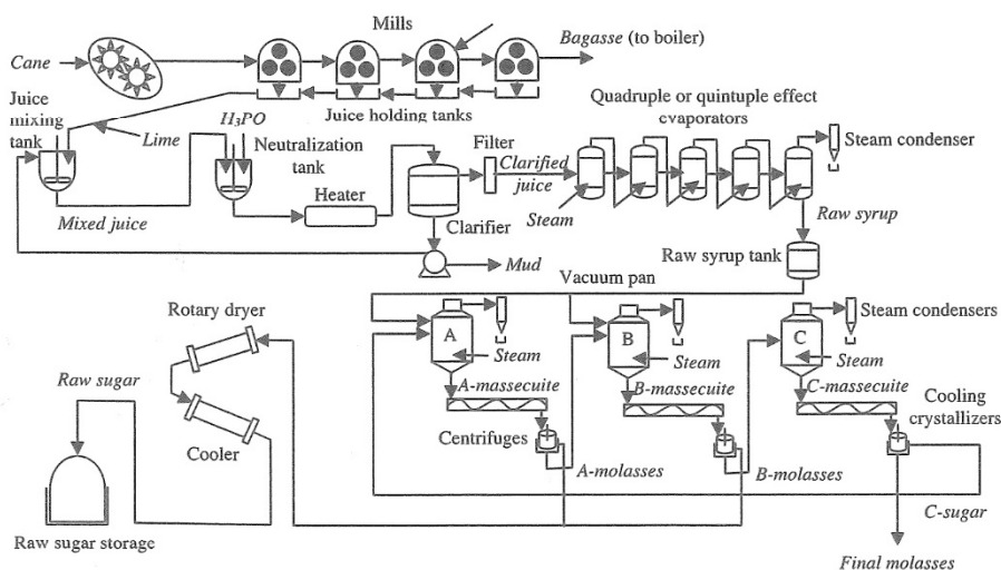
Figure 1. Flow chart for the raw sugar manufacturing process (Austin, 1984; Chen and Chou, 1993; The Energy Conservation Center, 2005). Process streams are named using italic font, and equipment with non italic font. Some auxiliary equipment has been omitted for clarity
