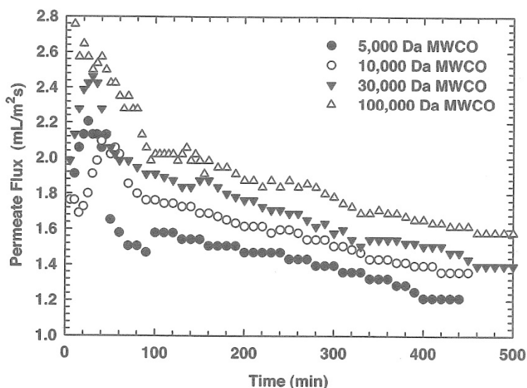
Figure 4. Changes in the permeate flux of mixed juice (prior to lime and heat treatment) through regenerated cellulose membranes as a result of membrane fouling
