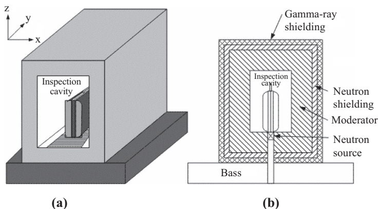
Figure 1. Simulation model of the EDS: (a) three dimensional view showing a briefcase inside the inspection cavity, (b) front view showing components of the EDS and layers of the EDS's walls
