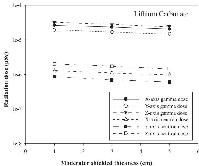
Figure 7. Semi-logarithmic plots of gamma ray and neutron doses as a function of \text{Li}_2\text{CO}_3 thickness at outer surfaces of the EDS's walls in X, Y, and Z directions when using polyethylene as a moderator
