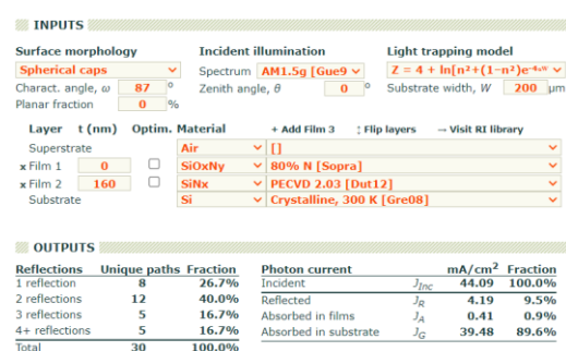
Figure 2. Parameters setting for OPAL 2 freeware
