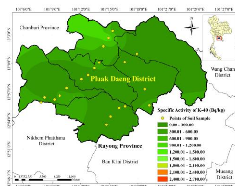
Figure 4. Radioactive Contour Maps (RCM) of ^{40}\text{K} in surface soil samples of Pluak Daeng district in Rayong Province
