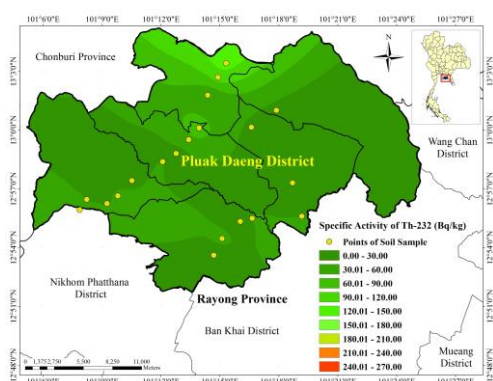
Figure 3. Radioactive Contour Maps (RCM) of ^{232}\text{Th} in surface soil samples of Pluak Daeng district in Rayong Province
