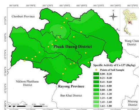
Figure 5. Radioactive Contour Maps (RCM) of ^{137}\text{Cs} in surface soil samples of Pluak Daeng district in Rayong Province
