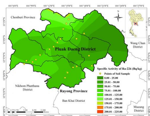
Figure 2. Radioactive Contour Maps (RCM) of ^{226}\text{Ra} in surface soil samples of Pluak Daeng district in Rayong Province
