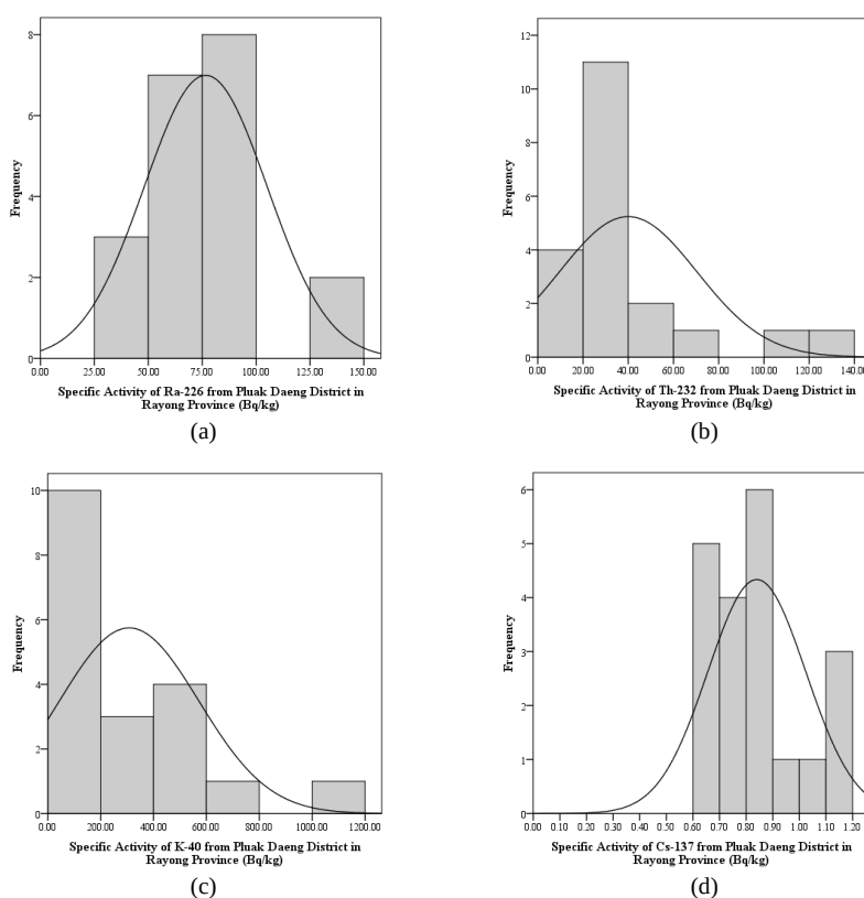
Figure 1. Frequency distribution of specific activities of (a) ^{226}Ra ; (b) ^{232}Th ; (c) ^{40}K and (d) ^{137}Cs in 20 surface soil samples collected from Plauk Daeng district in Rayong province
