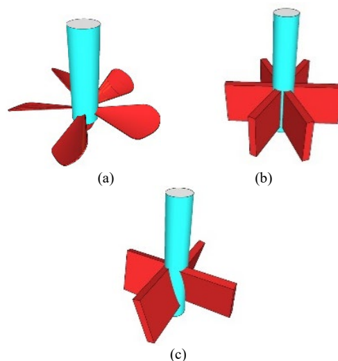
Figure 3. Different configuration impellers: 6-blade marine a) 6-straight-blade b) and 4-pitched-blade 30°
