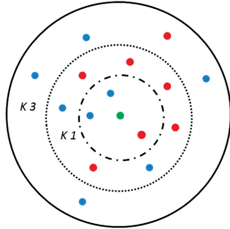
Figure 2. A representation of a KNN algorithm. The green dot represents the target whereas the red and blue dots represent 2 different classes based on the training set. 2 dashed circles represent the value of K in which the inner circle is equal to 1 and the outer dashed circle is 3
