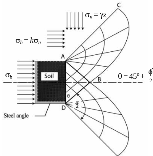
Figure 3. Possible failure mechanism of a single isolated transverse member (Horpibulsuk and Niramitkornburee, 2010)
