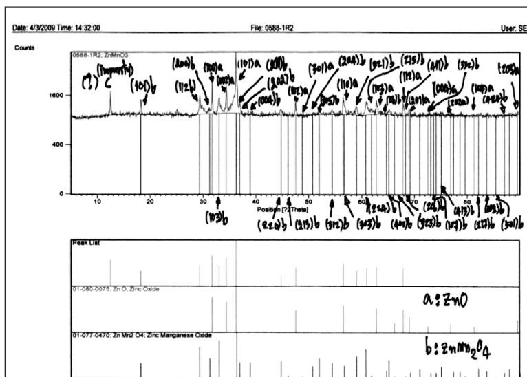
Figure 5. XRD pattern at room temperature for \text{ZnO-ZnMn}_2\text{O}_4 ceramics
