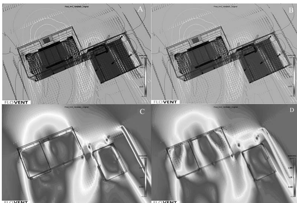
Figure 6. Wind field distribution in different height interfaces (a) H = 0.8 , (b) H = 1.60 (c) H = 3.65 , (d) H = 4.45
