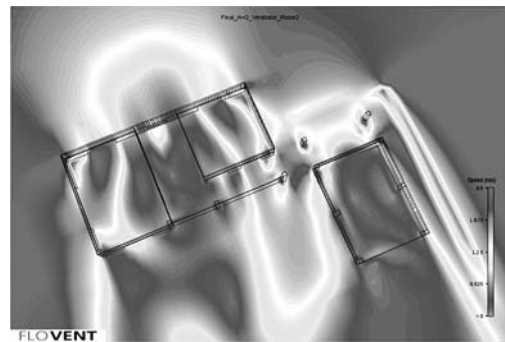
Figure 10. Wind field distribution after modify the design by adding a small bedroom (H = 4.45 m)
