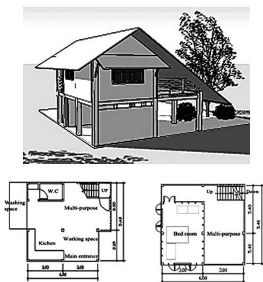
Figure 1. Floor plans and interior view of primary structure
