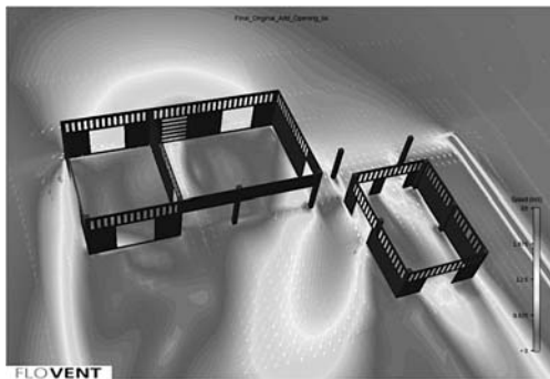
Figure 9. Wind field distribution after adding a window in the west room (H = 3.65 m)
