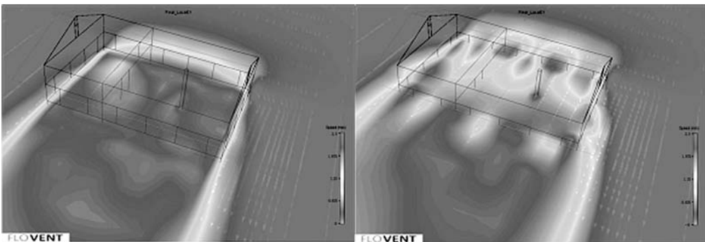
Figure 8. Wind field distribution in conventional dwelling H = 3.65 m (Left), H = 4.45 m (right)
