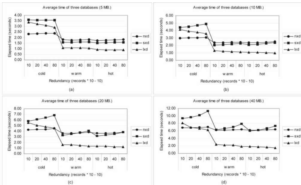
Figure 3. Average time of nxd, sxd, and lxd in cold, warm, and hot caches nxd: native XML database; sxd: single XML document database; lxd: linked XML document database
