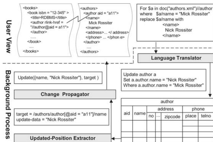
Figure 1. Overview of the solution to updating XML documents
