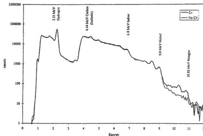
Figure 3. Gamma ray spectrum resulting from inspection of 300 g of C-4, using ^{241}\text{Am}/^9\text{Be} (Gozani, 1996)
