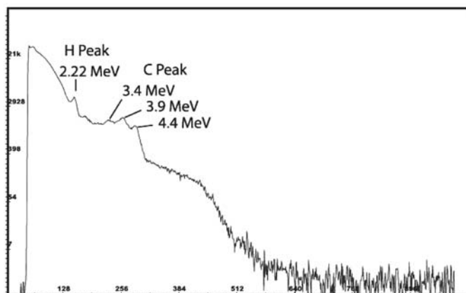
Figure 5. The gamma ray spectrum resulting from inspection of TNT of 1,000 g for 900 s, using ^{241}\text{Am}/^9\text{Be} , in which the 4.4-MeV gamma rays with their single and double escapes of energies of 3.9 and 3.4 MeV, respectively, are observed in the spectrum
