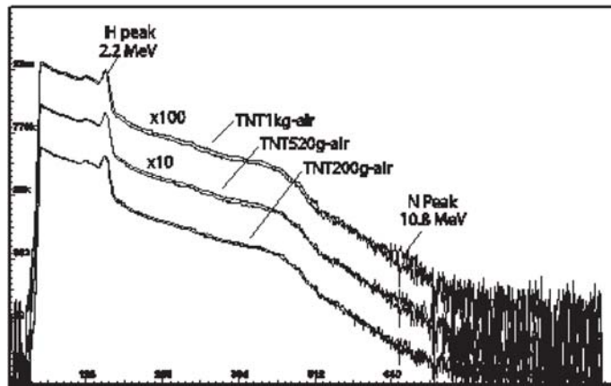
Figure 2. Gamma ray spectra resulting from inspection of 1,000, 520, and 200 g of TNT in the inspection cavity using ^{252}\text{Cf} for 900 s
