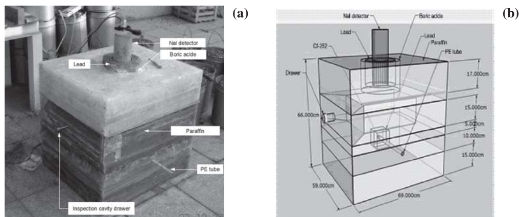
Figure 1. Experimental set-up: (a) photograph and (b) three dimensional drawing showing locations and dimensions of its components
