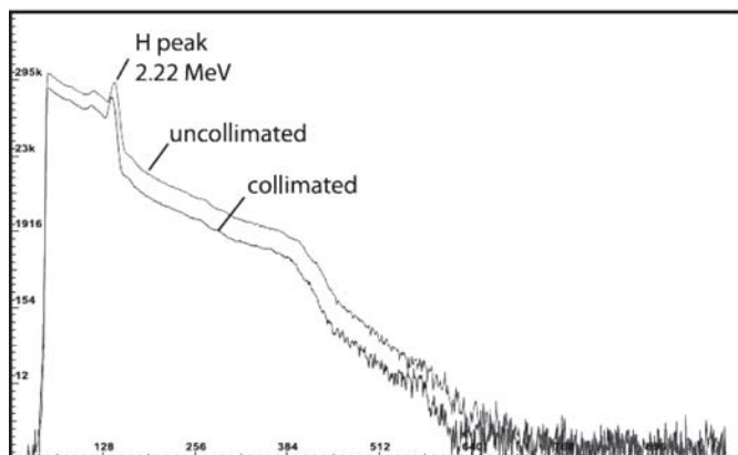
Figure 4. A comparison between gamma-ray spectra resulting from inspection of 1,000 g of TNT using the collimated and un-collimated gamma-ray detectors
