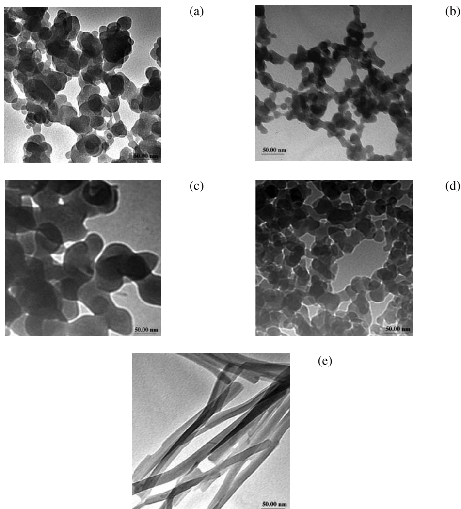
Figure 1. TEM micrographs of the \text{Ce}_{0.8}\text{Sm}_{0.2}\text{O}_{2-\delta} synthesized by using different mole ratios (R) and reaction temperatures (T) (50,000X): (a) R = 6.67, T = 70°C, (b) R = 10, T = 70°C, (c) R = 10, T = 50°C, (d) R = 10, T = 29°C, (e) R = 13.33, T = 70°C
