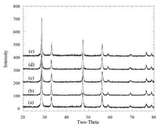
Figure 2. XRD patterns of \text{Ce}_{0.8}\text{Sm}_{0.2}\text{O}_{2-\delta} synthesized via different synthesis conditions after calcination at 800^\circ\text{C} : (a) R = 6.67 , T = 70^\circ\text{C} , (b) R = 10 , T = 70^\circ\text{C} , (c) R = 10 , T = 50^\circ\text{C} , (d) R = 10 , T = 29^\circ\text{C} , (e) R = 13.33 , T = 70^\circ\text{C}
