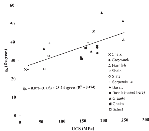
Figure 6. Basic friction angles as a function of UCS for various rock types obtained elsewhere (Waltham, 1994; Geasselli and Eggar, 2002)
