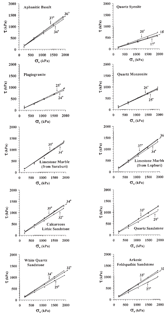
Figure 3. Results of direct shear testing on saw cut surfaces of ten rock types
