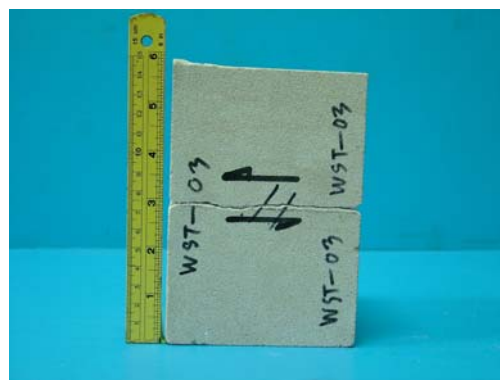
Figure 8. Quartz sandstone specimens with tension-induced fracture prepared for direct shear testing. Arrows indicate shear direction.
