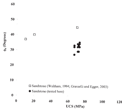
Figure 5. Basic friction angles as a function of UCS for sandstones
