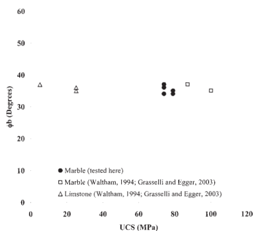
Figure 4. Basic friction angles as a function of UCS for marbles and limestone
