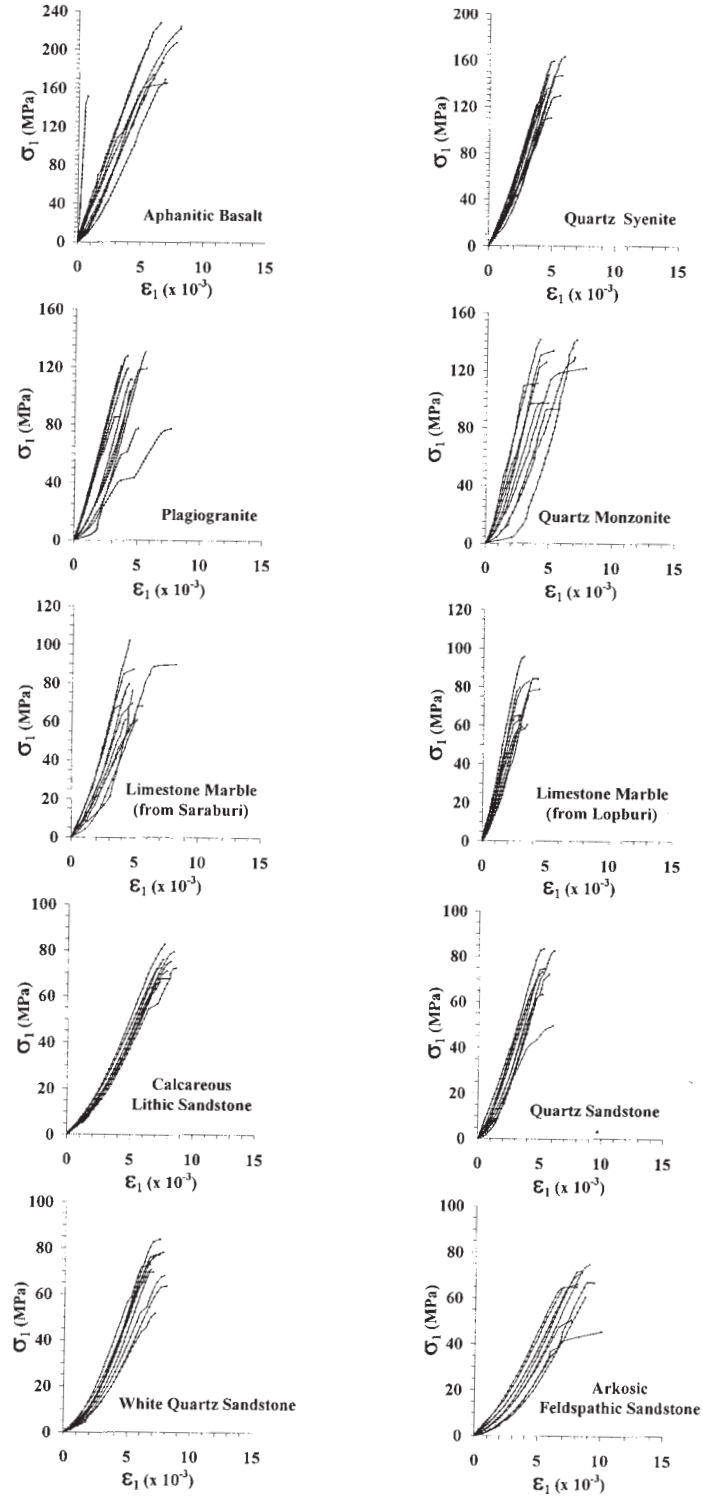
Figure 1. Results of uniaxial compressive strength testing from ten rock types
