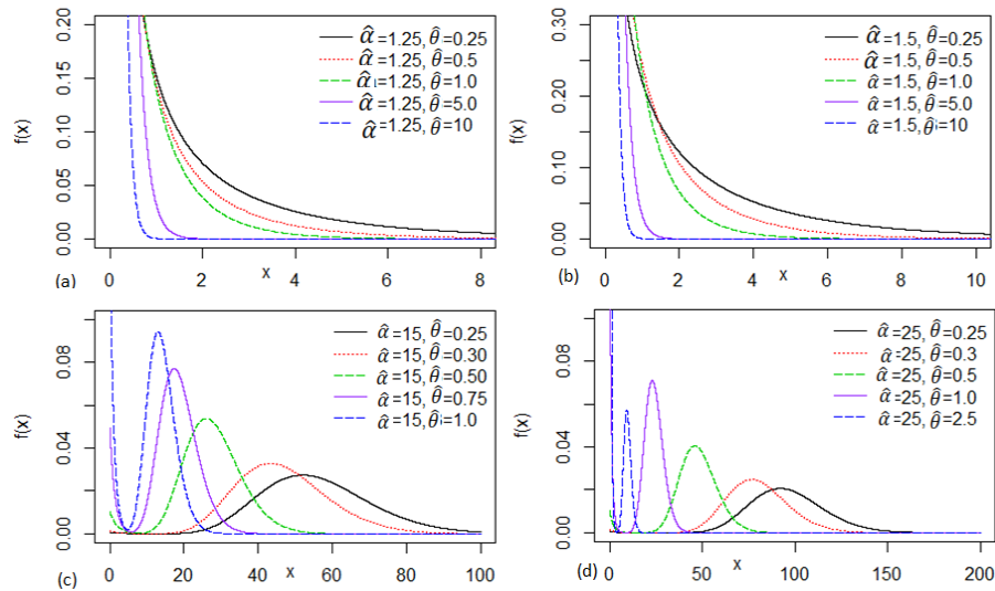
Figure 1. The probability density curves for various selected values of the shape and scale parameters
