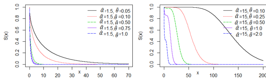
Figure 3. Survival curves of the distribution for some selected values of parameters
