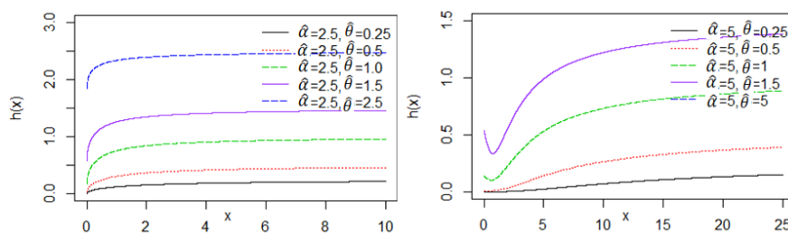
Figure 4. Hazard curves of the distribution for some selected values of parameters
