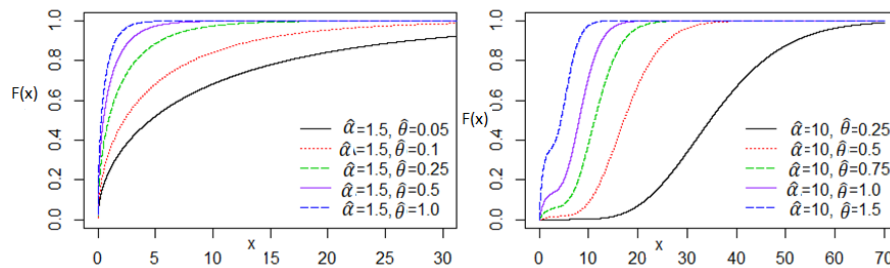
Figure 2. CDF curves of the EG-L distribution for some selected values of parameters
