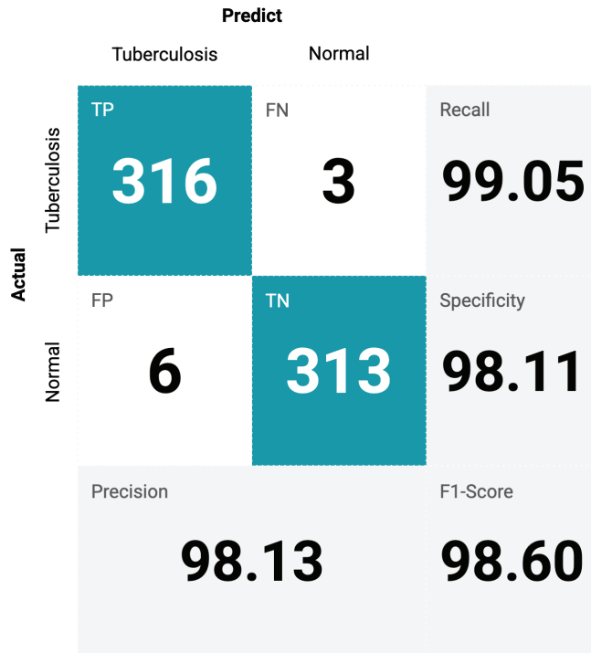
Figure 7 Confusion Matrix Best Model (VGG16 + FC Pattern 11)
