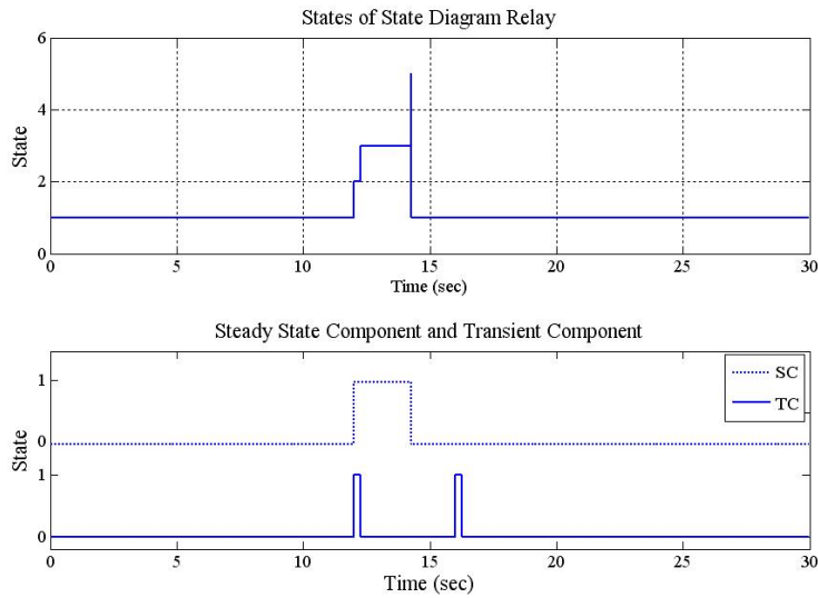
Figure 7 State transition of SDR under short-circuit fault
