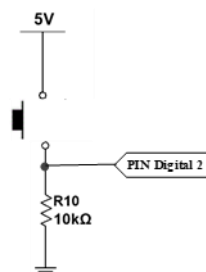
Figure 2 Switch Control Circuit
