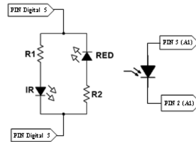
Figure 1 Sensor Circuit
