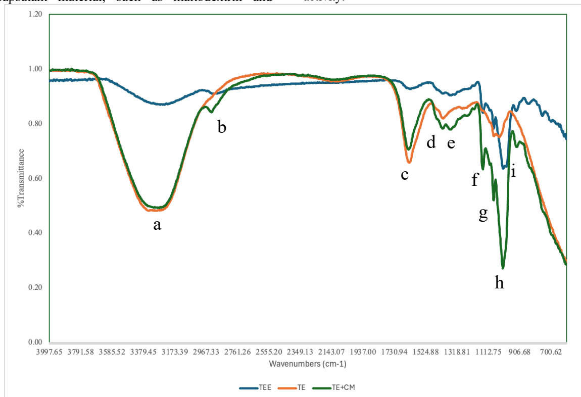
Figure 2. FTIR spectra of TEE (Tiwai Extract Encapsulant), TE (Tiwai Extract), TE+CM (Tiwai Extract + Coating Material) scanned at wave numbers 4000–650 \text{cm}^{-1} using the damped total reflectance (ATR) mode
