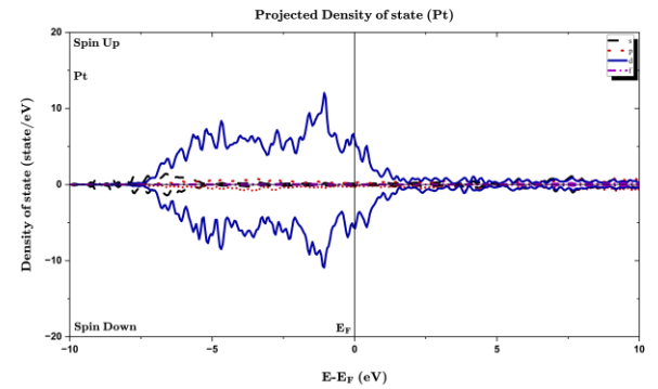
Fig. 8 Spin-polarized PDOS for Pt layers from Co/Pt structure
