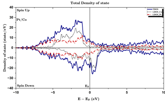
Fig. 3 Spin-polarized TDOS for the Co and Pt layers (Co/Pt)
