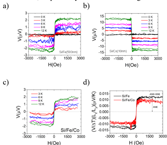
Fig.12 The magnetic field ( H ) dependence a) Fe(500nm) b) Co(10nm) c) Fe(500nm)/Co(10nm) d) The normalized voltage ( E/IT ) of Fe(500) and Fe(500)/Co(10)
