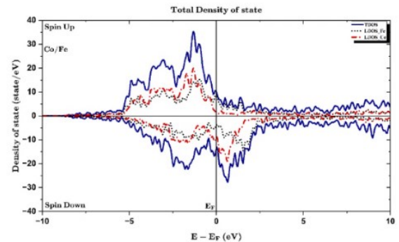
Fig. 1 Spin-polarized TDOS for the Fe and Co layers (Fe/Co)
