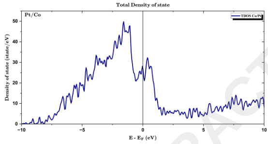
Fig. 4 TDOS for the Co and Pt layers (Co/Pt)
