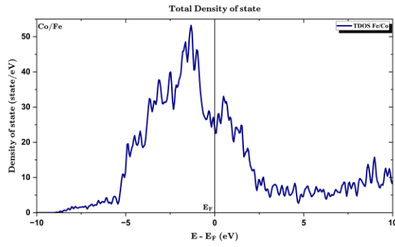
Fig. 2 TDOS for the Fe and Co layers (Fe/Co)
